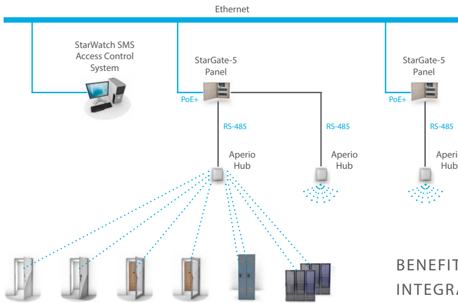
Each StarGate-5 supports up to 16 locks, which can be distributed across up to 8 Aperio wireless hubs, each supporting up to 8 locks.
